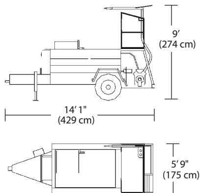
T60T TRAILER
